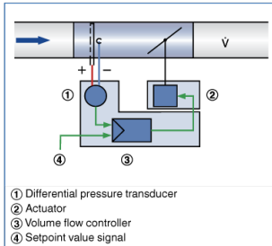
Principle of operation – Universal TROX/ Gruner
